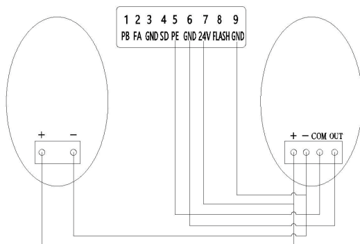
Connection of photo beam/switch control
